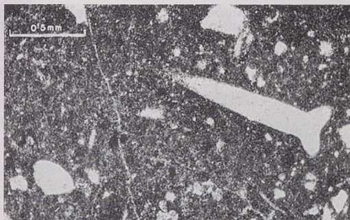
Plate 1: Sponge spicules from Poh Kwong Quarry (de Coo and Lau, 1977, p. 75).
