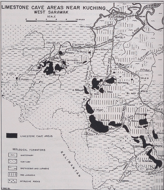
Figure 1: Map of limestone near Kuching, showing geological formations (from Wilford, 1964, Figure 18).
